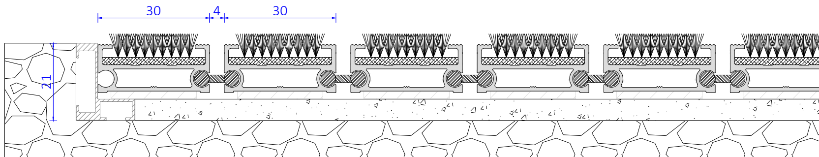
Vertical cross section mat
