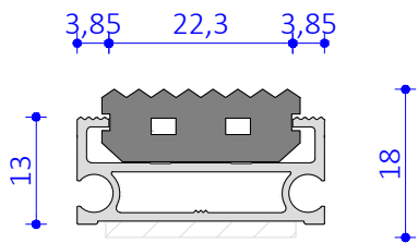
Detail with inlay rubber
